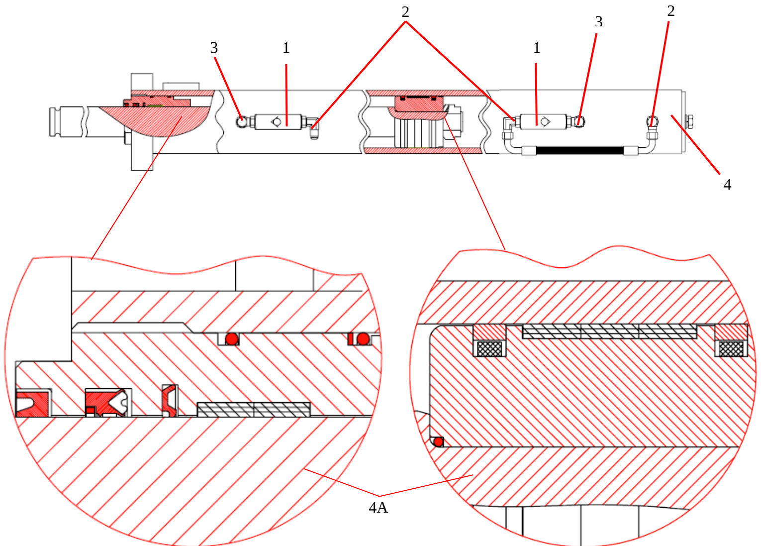
73120A-SK SEAL KIT ASSEMBLY
