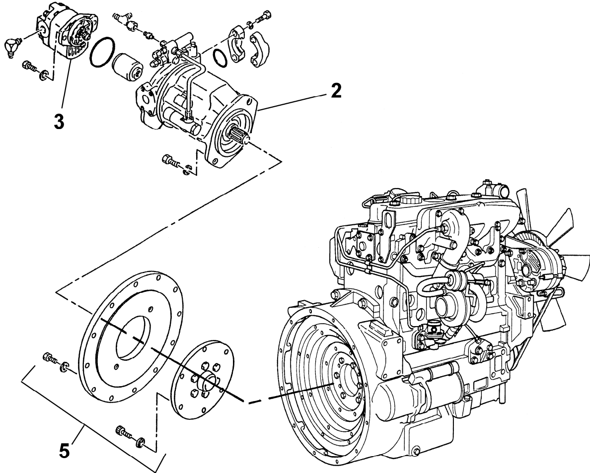
PERKINS DIESEL ENGINE BW10039-2 (REF)
